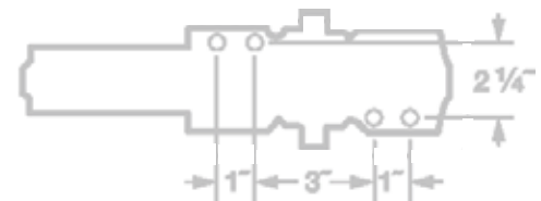
Hole Pattern
